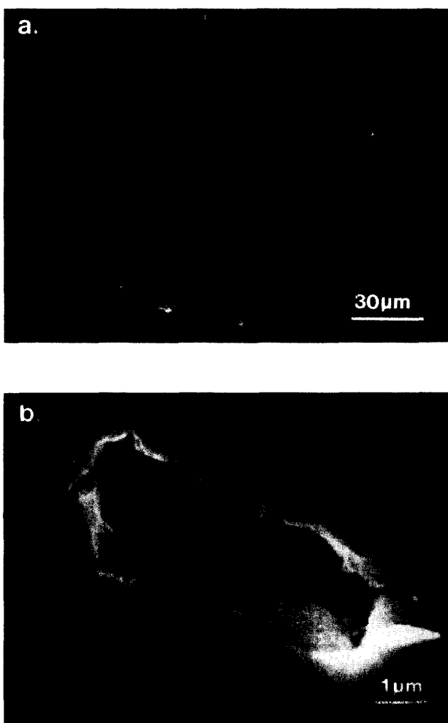
Fig. 3. SEM micrographs taken from the low N-containing steel after polarization to 800 mV for 2 h.
